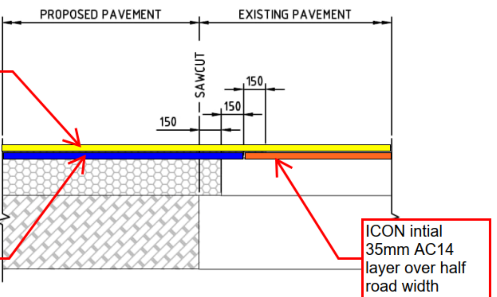
PAVEMENT INTERFACE DETAIL
