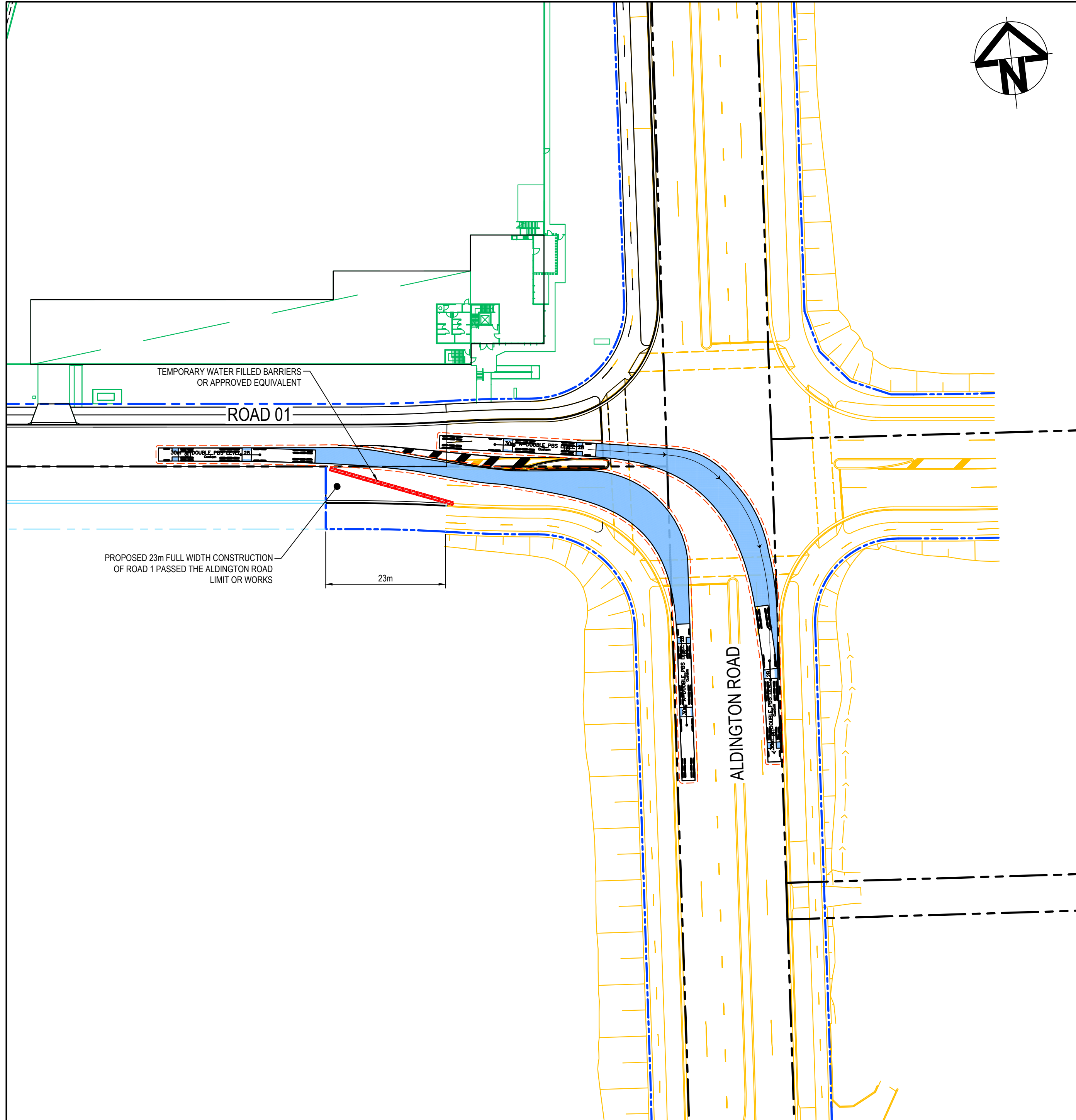
30m B-DOUBLE PBS LEVEL 2 TRUCK ENTRY/EXIT
