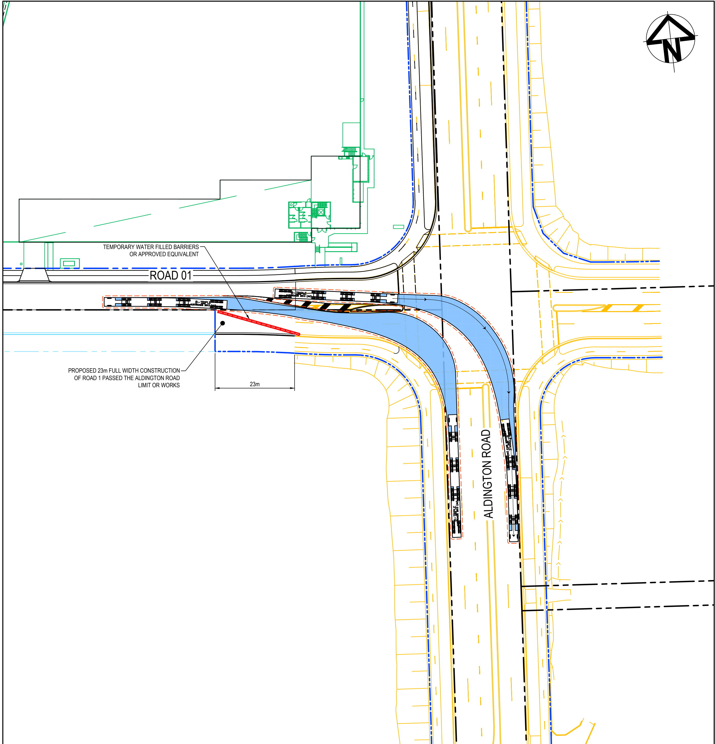
36.5m B-TRIPLE TRUCK ENTRY/EXIT
