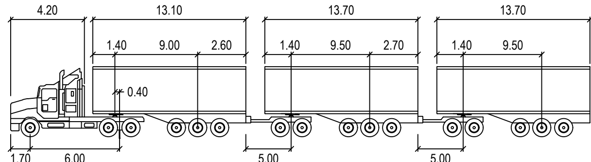
36.5m B-TRIPLE
